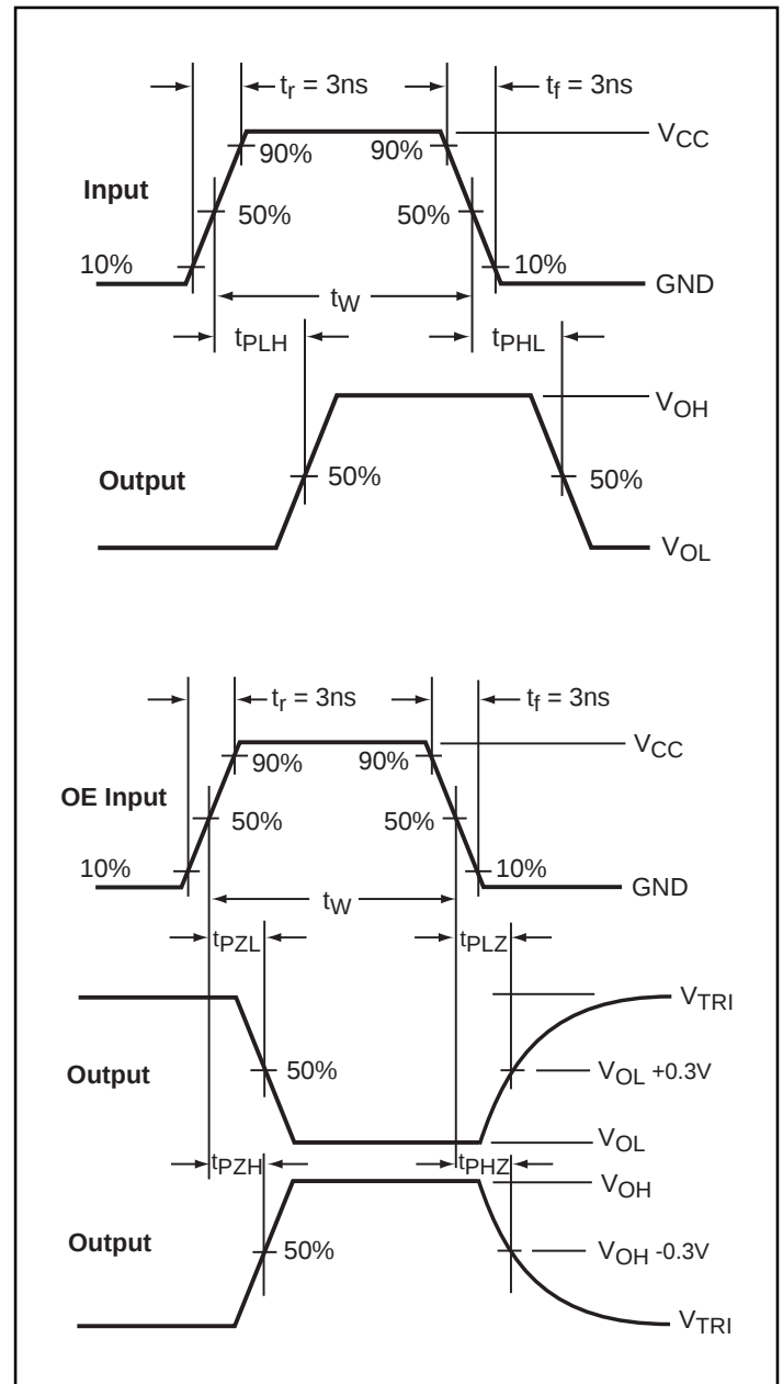
Figure 3. AC Waveforms
