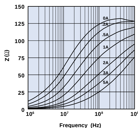
Figure 17B Impedance vs. frequency with dc bias as parameter for bead on lead 2743002112.
