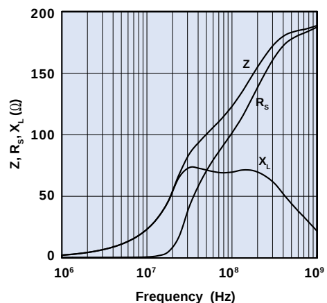
Figure 21A Impedance, reactance, and resistance vs. frequency for bead on lead 2761007112.
