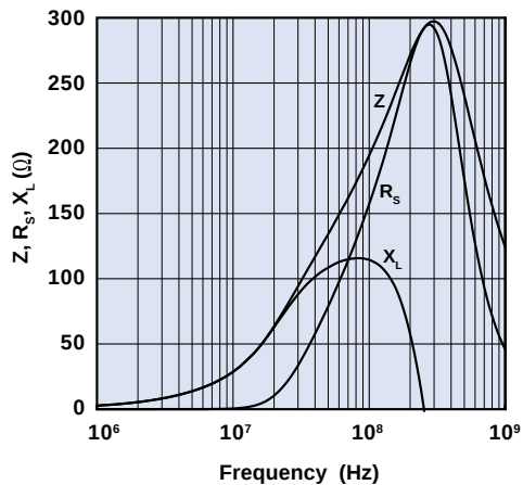
Figure 18 Impedance, reactance, and resistance vs. frequency curve for multi-aperture core 2861001702.
