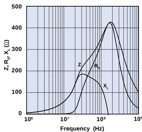
Figure 33 Impedance, reactance, and resistance vs. frequency curve for multi-aperture core 2861006802.
