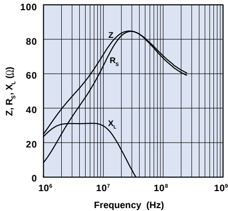
Figure 10A Impedance, reactance, and resistance vs. frequency for bead on lead 2773003112.
