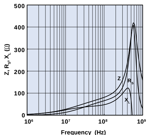
Figure 11 Impedance, Reactance, and Resistance vs. Frequency for 43 material split round cable EMI suppression core 2643806406.
