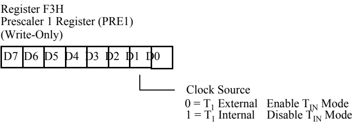
Figure 6-14. Prescaler 1 Register (T IN Operation)
