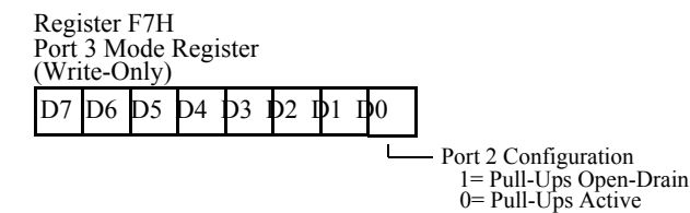
Figure 5-34. Port 2 Configuration
