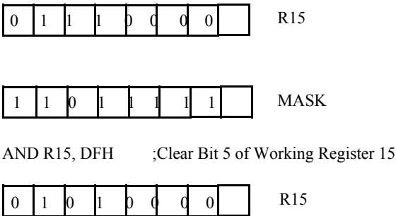
Figure 2-2. Accessing Individual Bits (Example)
