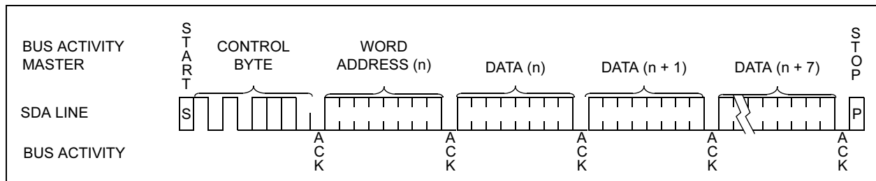
FIGURE 4-2: PAGE WRITE
