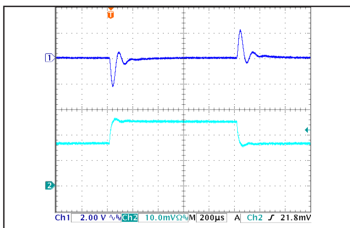
Figure 5: Output voltage response to step-change in load current (66%-100%-66% of Iout(max); dI/dt = 0.1A/μs). Load cap: 1μF ceramic cap. Ch 1: Vout, Ch 2: Iout (1 A/div).
