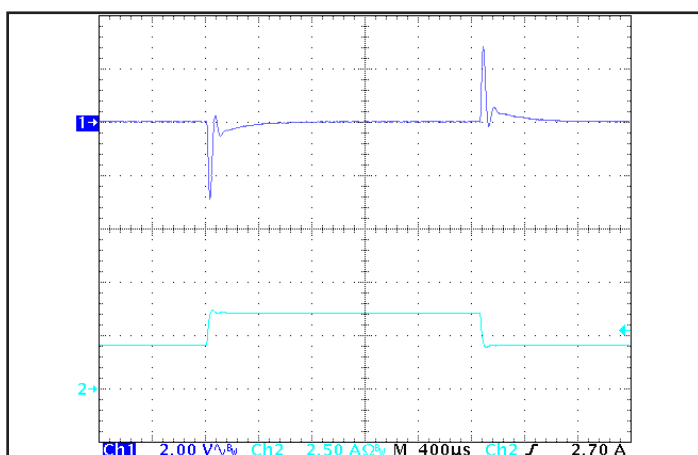
Figure 5: Output voltage response to step-change in load current (66%-100%-66% of I out (max); dI/dt = 0.1A/μs). Load cap: 1μF ceramic cap. Ch 1: V out , Ch 2: I out .
