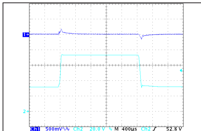
Figure 6: Output voltage response to step-change in input voltage (V nom. -V max -V nom. ), at Max. load current. Load cap: 15μF tantalum capacitor and 1μF ceramic cap. Ch 1: V out , Ch 2: V in .
