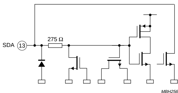
Fig.28 Simplified circuit diagram pin 13.
