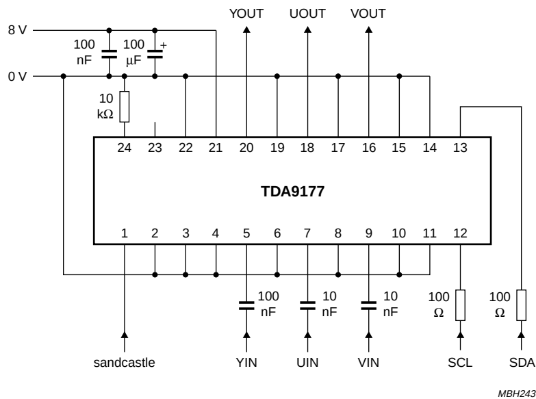
Fig.40 Application diagram.
