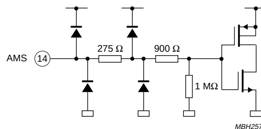
Fig.29 Simplified circuit diagram pin 14.
