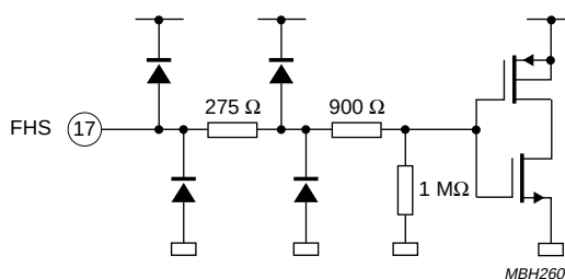
Fig.32 Simplified circuit diagram pin 17.
