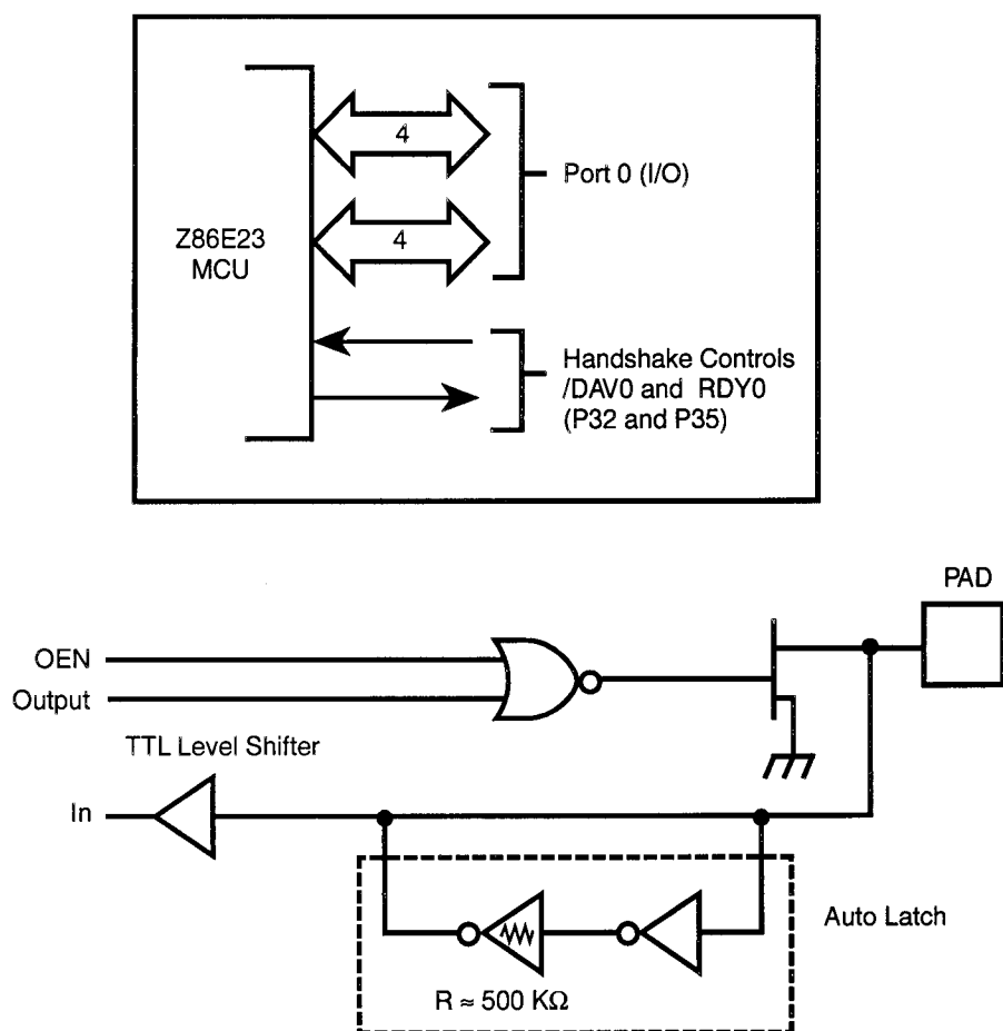
Figure 8. Port 0 Configuration
