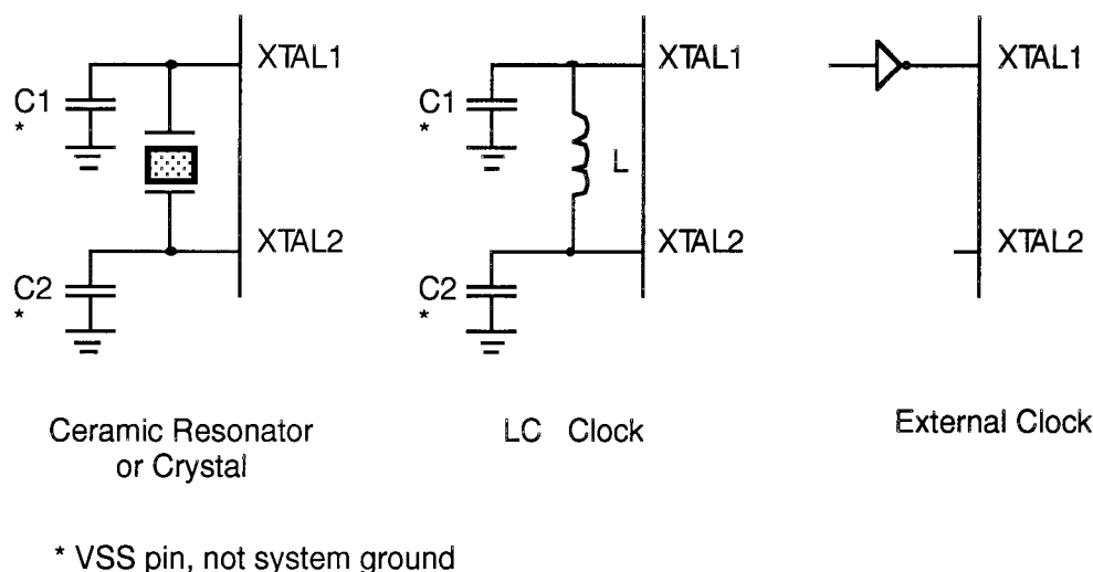
Figure 17. Oscillator Configuration
