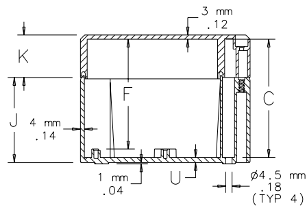
SECTION C-C
