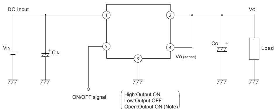
Fig.19 Typical Application
