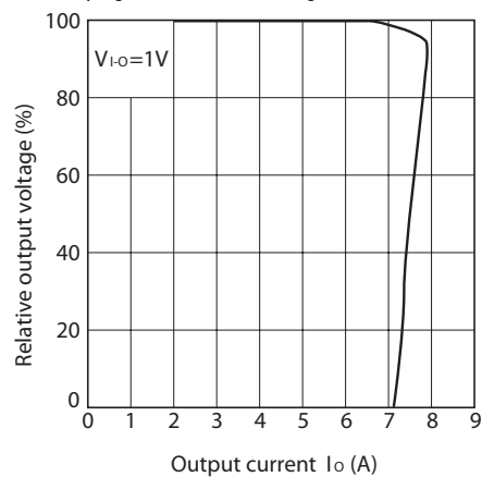
Fig.5 Overcurrent Protection Characteristics (PQ015Y053ZxH / PQ025Y053ZxH / PQ033Y053ZxH)
