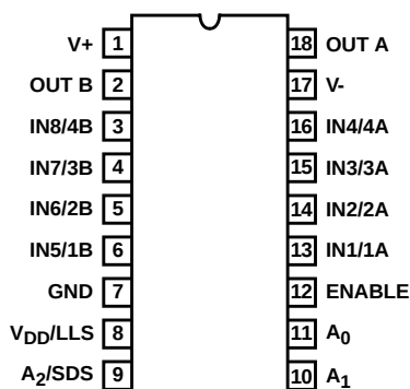
HI-518 (CERDIP, PDIP) TOP VIEW
