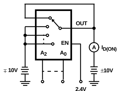
FIGURE 4. I_{D(ON)} (NOTE 1)
