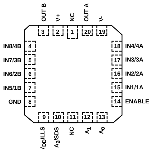
HI-518 (CLCC, PLCC) TOP VIEW
