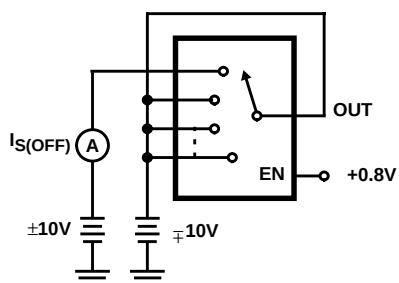
FIGURE 3. I_{S(OFF)} (NOTE 1)
