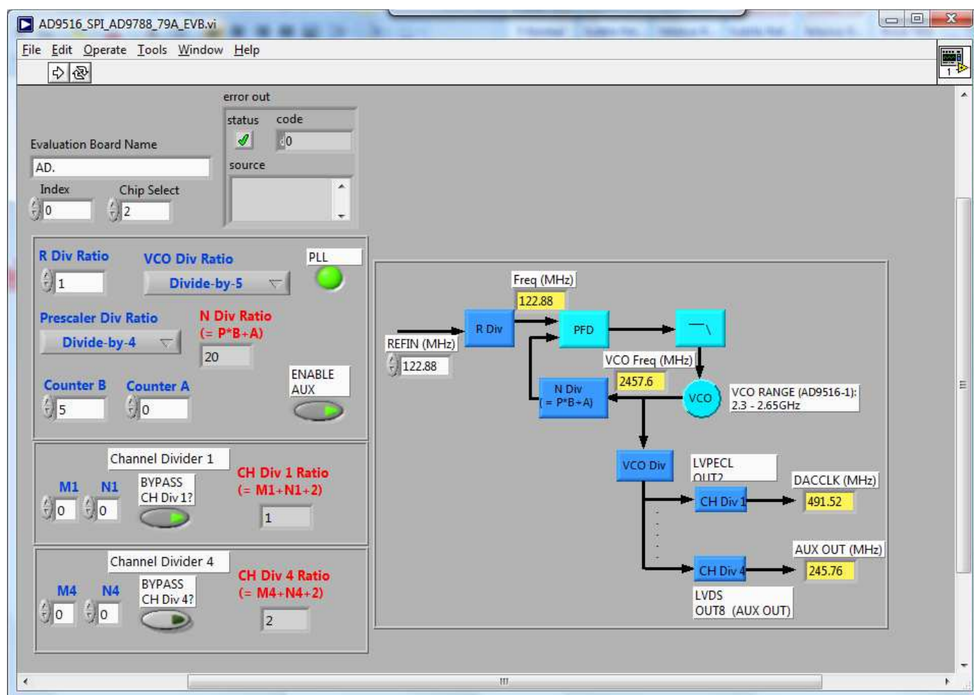
Figure 11 AD9516 SPI Control
