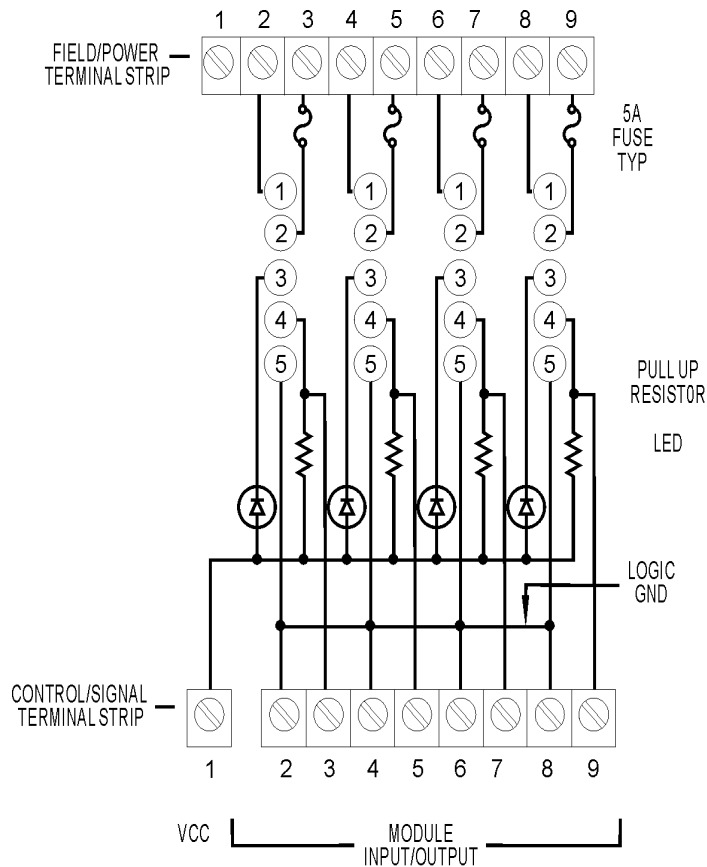
PB4 SCHEMATIC
