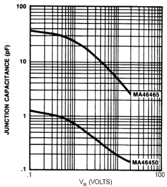
JUNCTION CAPACITANCE vs REVERSE BIAS VOLTAGE (γ = 1.0) (CHIPS)
