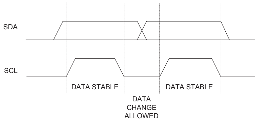
Figure 5-3. Data Validity
