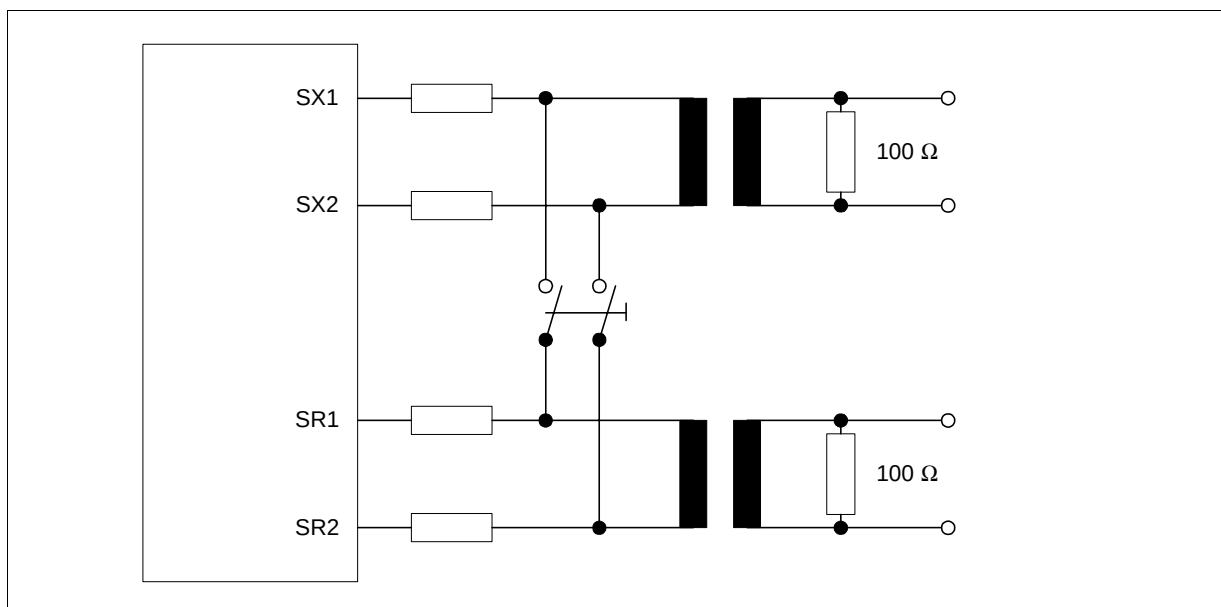
Figure 27 External Loop at the S/T-Interface
