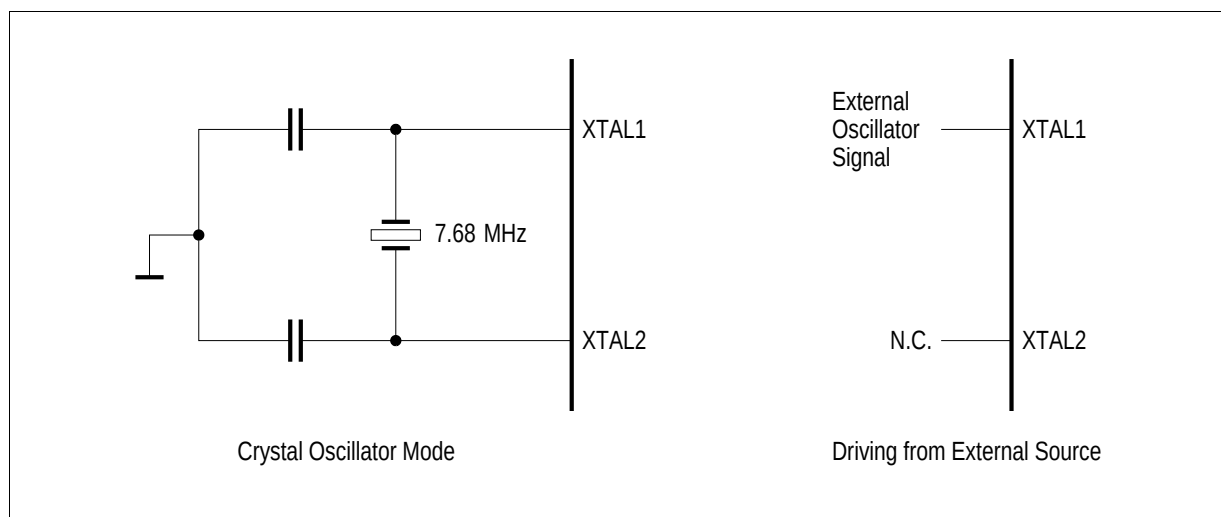
Figure 67 Oscillator Circuits
