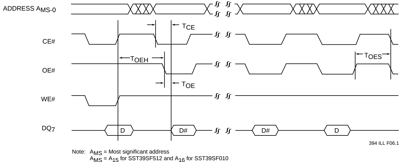
FIGURE 7: DATA# POLLING TIMING DIAGRAM
