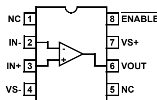
EL8186 (8-PIN SO) TOP VIEW
