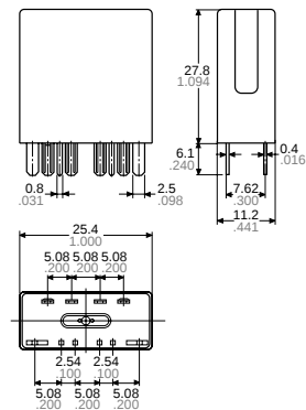
External dimensions
