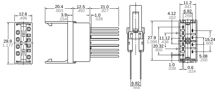
External dimensions
