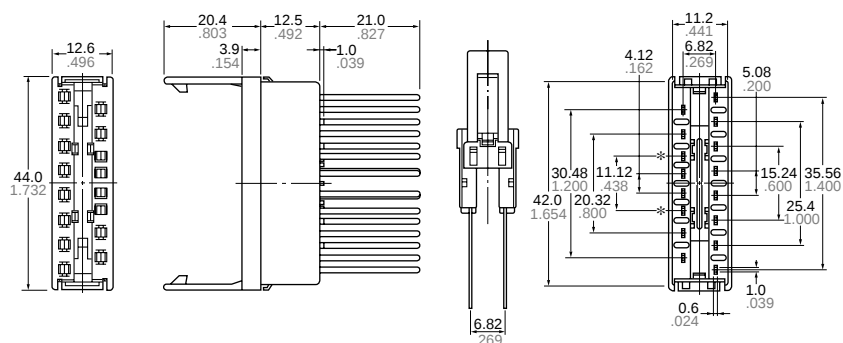
External dimensions
