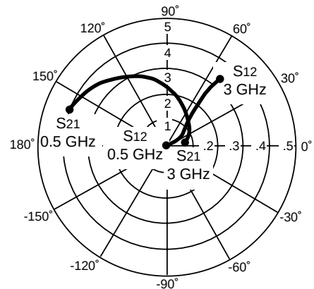
Coordinates in Ohms Frequency in GHz (V CE = 2.5 V, I C = 2.5 mA)
