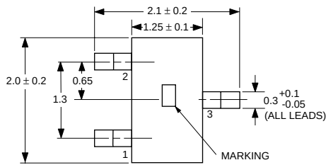
PACKAGE OUTLINE 30
