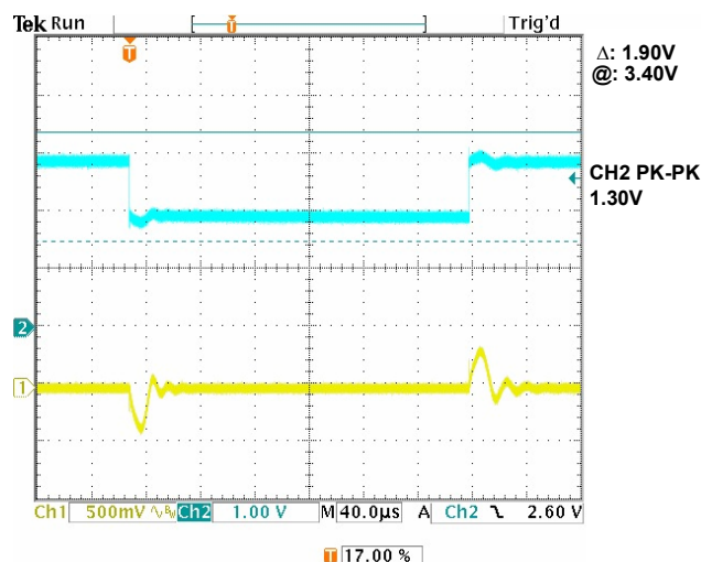
FIGURE 43. LOAD TRANSIENT RESPONSE, 100nF LOAD CAPACITANCE
