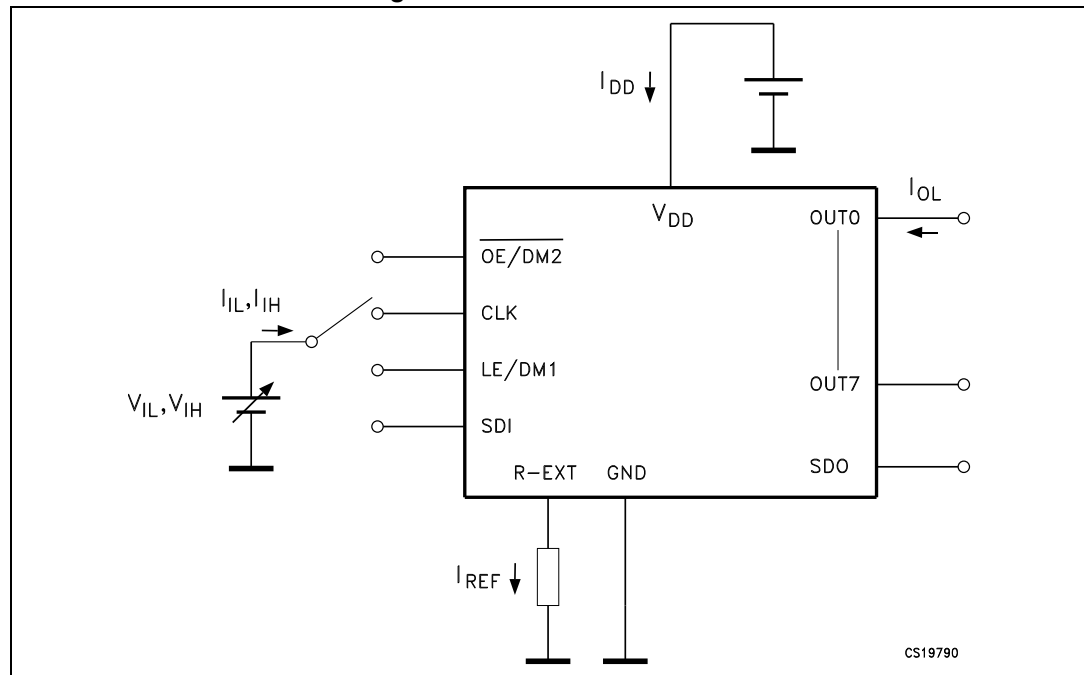
Figure 14. DC characteristics
