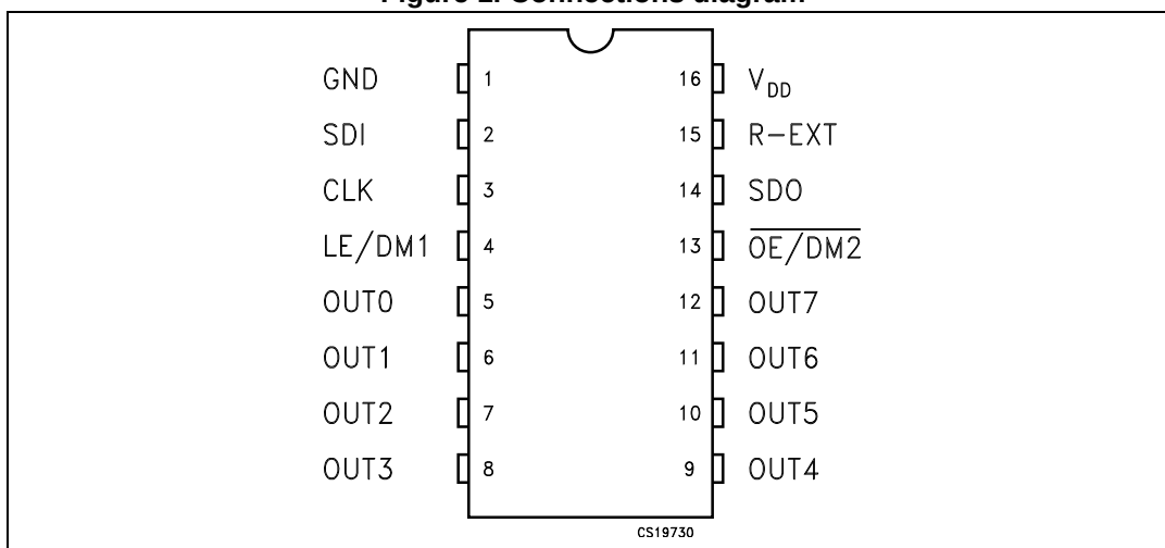
Figure 1. Connections diagram
