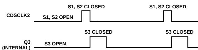
Figure 11. SHA-Mode Internal Switch Timing
