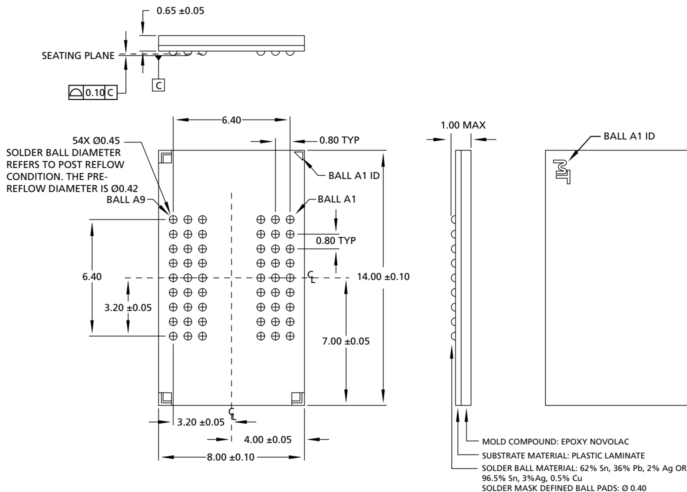
Figure 9: 54-Ball VFBGA "FG" (8mm x 14mm) (x16)
