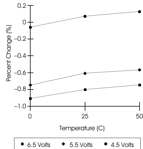
Graph 2-48: Oscillator Stability
