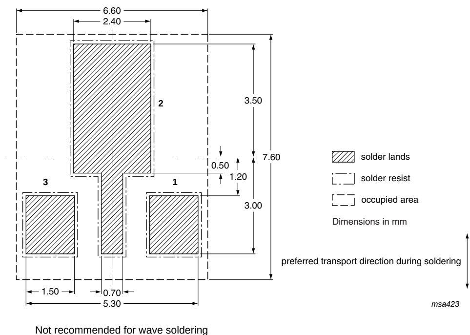
Fig 17. Wave soldering footprint SOT89 (SC-62)
