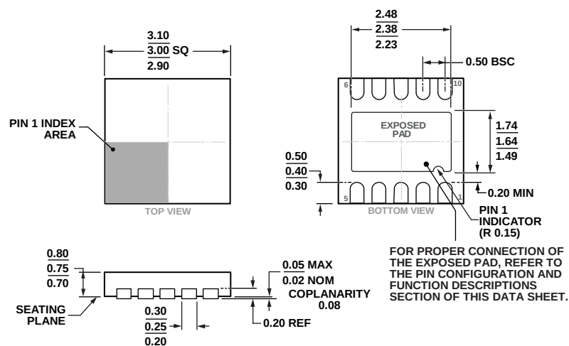
Figure 45. 10-Lead Lead Frame Chip Scale Package [LFCSP_WD] 3 mm × 3 mm Body, Very Very Thin, Dual Lead (CP-10-9)
