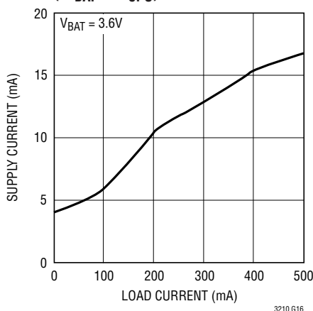
2x Mode Supply Current vs I_{CP0} ( I_{VBAT} = 2I_{CP0} )
