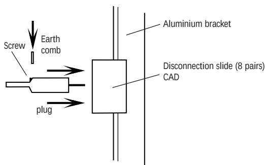
Module connection
