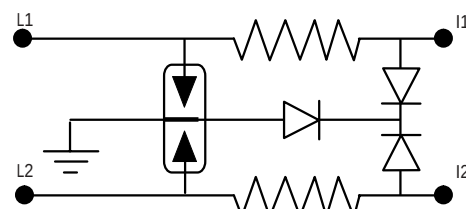
Series protection
