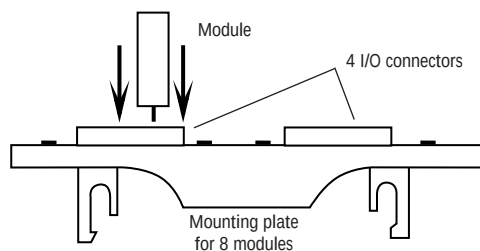
Module connection
