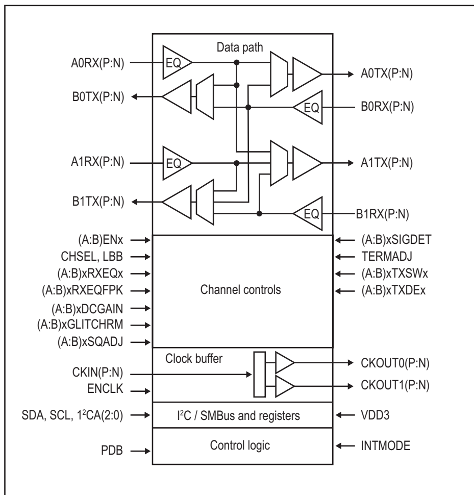
89HP0604R Block Diagram
