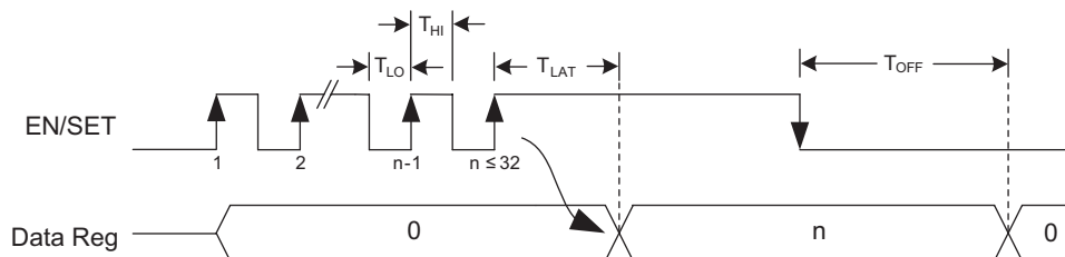
Figure 1: S 2 Cwire Timing Diagram.
