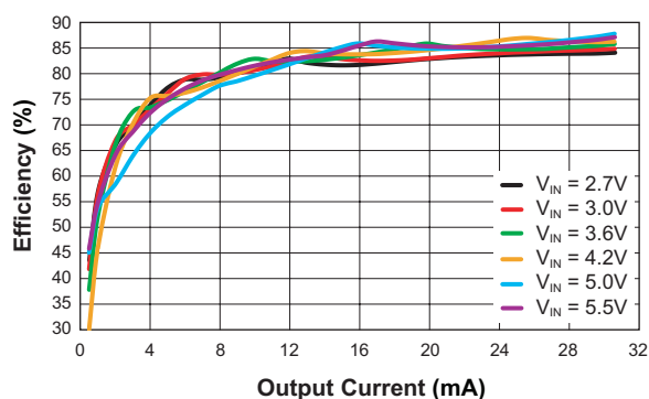
Efficiency vs. Output Current ( R_{SET} = 10k\Omega , L = 10\mu H , 4 LEDs)
