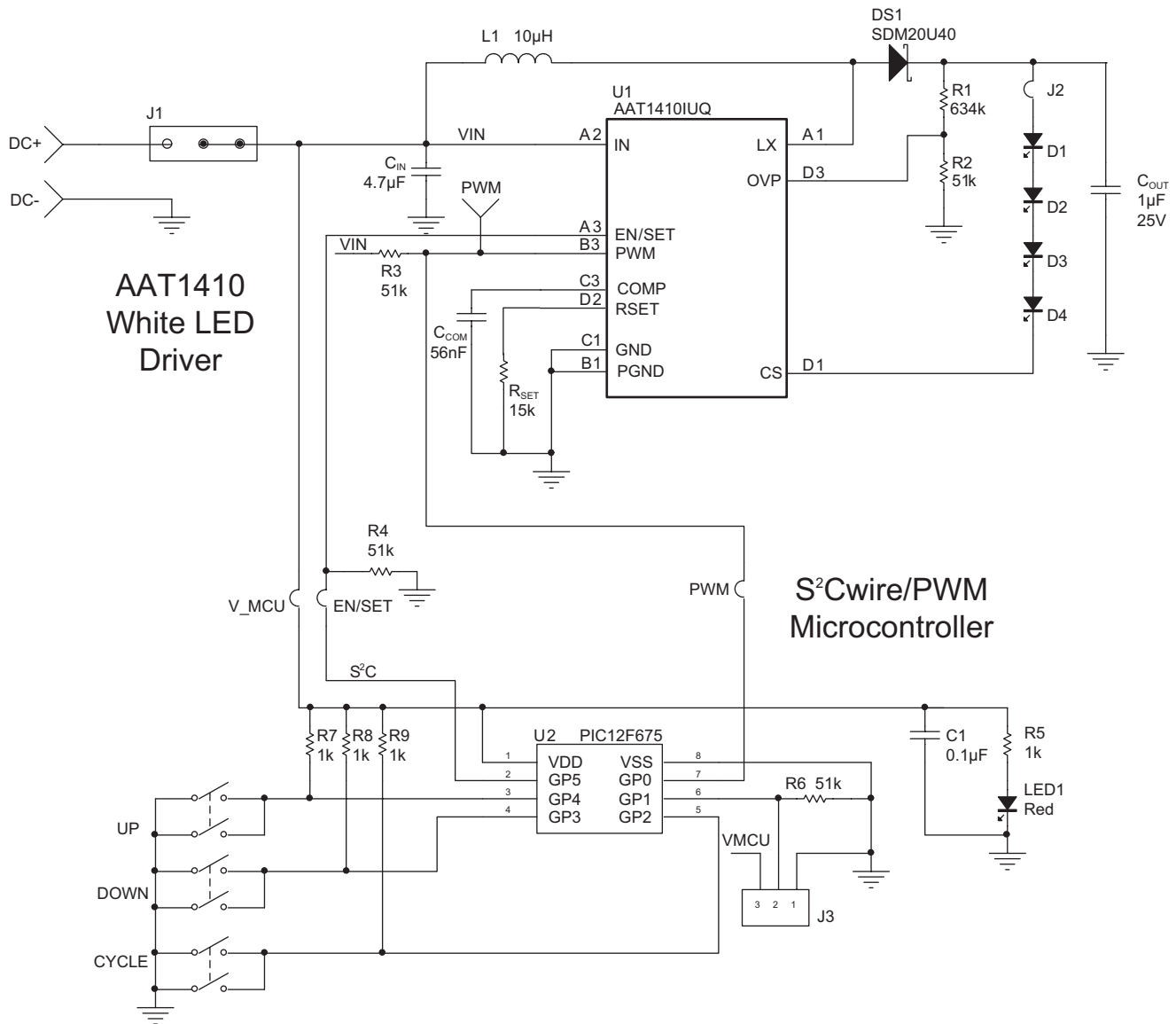
Figure 6: AAT1410 Evaluation Board Schematic.
