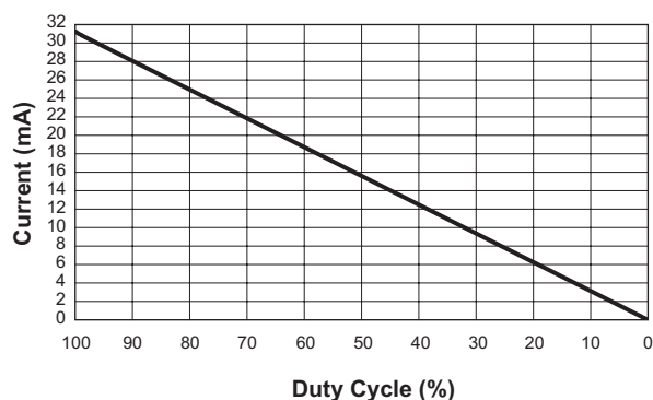
LED Current vs. PWM Duty Cycle ( V_{IN} = 3.6V , R_{SET} = 10K\Omega )
