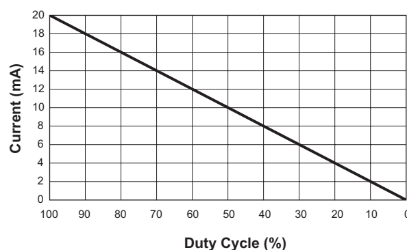
LED Current vs. PWM Duty Cycle ( V_{IN} = 3.6V , R_{SET} = 15K\Omega )
