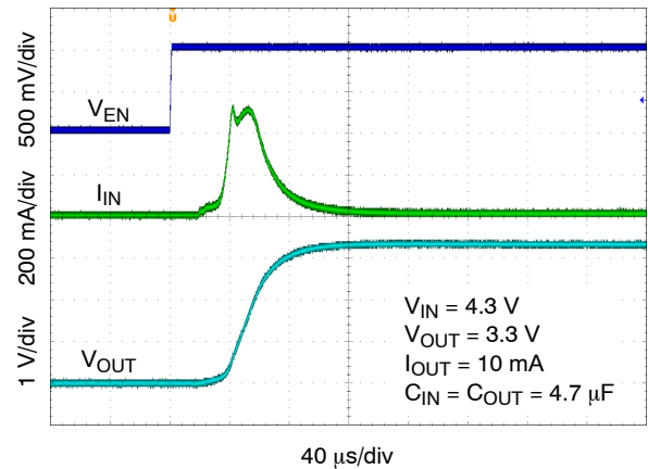
Figure 33. Enable Turn-on Response – V OUT = 3.3 V, C OUT = 4.7 μF
