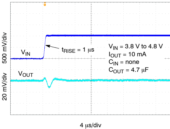
Figure 38. Line Transient Response– Rising Edge, V_{OUT} = 3.3\text{ V} , I_{OUT} = 10\text{ mA} , C_{OUT} = 4.7\text{ μF}
