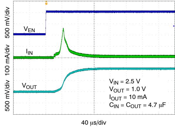
Figure 31. Enable Turn-on Response – V OUT = 1.0 V, C OUT = 4.7 μF
