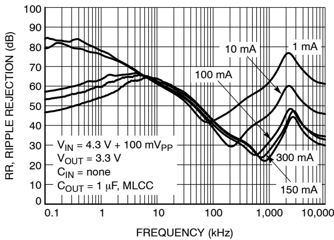
Figure 25. Power Supply Rejection Ratio, V_{OUT} = 3.3\text{ V}
