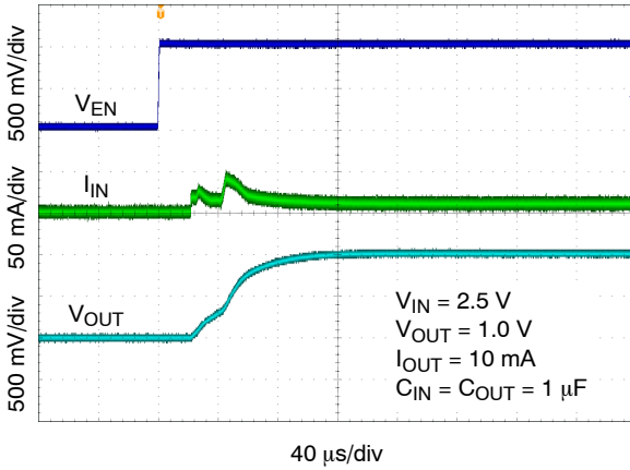
Figure 30. Enable Turn-on Response – V OUT = 1.0 V, C OUT = 1 μF
