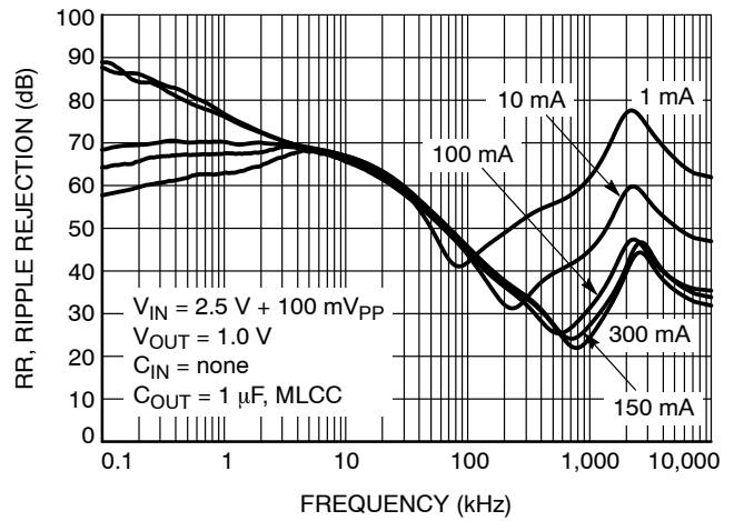
Figure 24. Power Supply Rejection Ratio, V_{OUT} = 1.0\text{ V}
