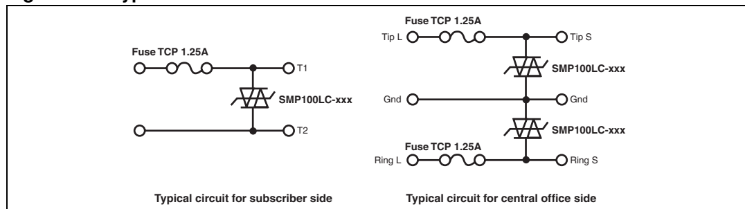
Figure 11. Typical circuits
