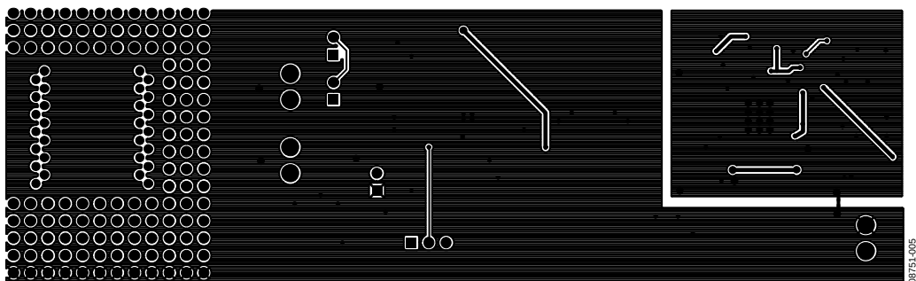
Figure 5. AD7171 Evaluation Board—Solder Side View
