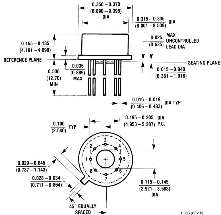
Metal Can Package (H) NS Package Number H08C
