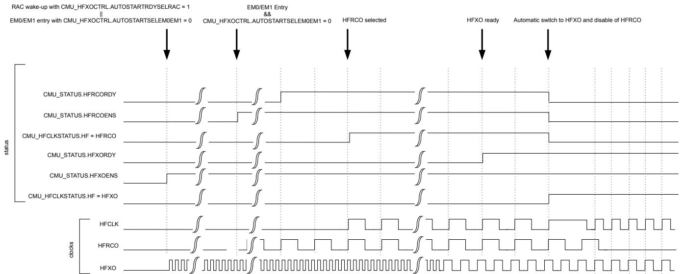
Figure 11.14. CMU HFRCO startup/selection while awaiting automatic HFXO startup/selection
