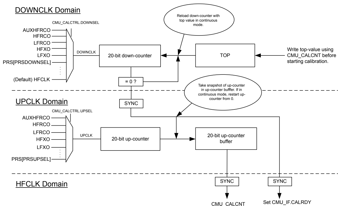
Figure 11.10. HW-support for RC Oscillator Calibration
