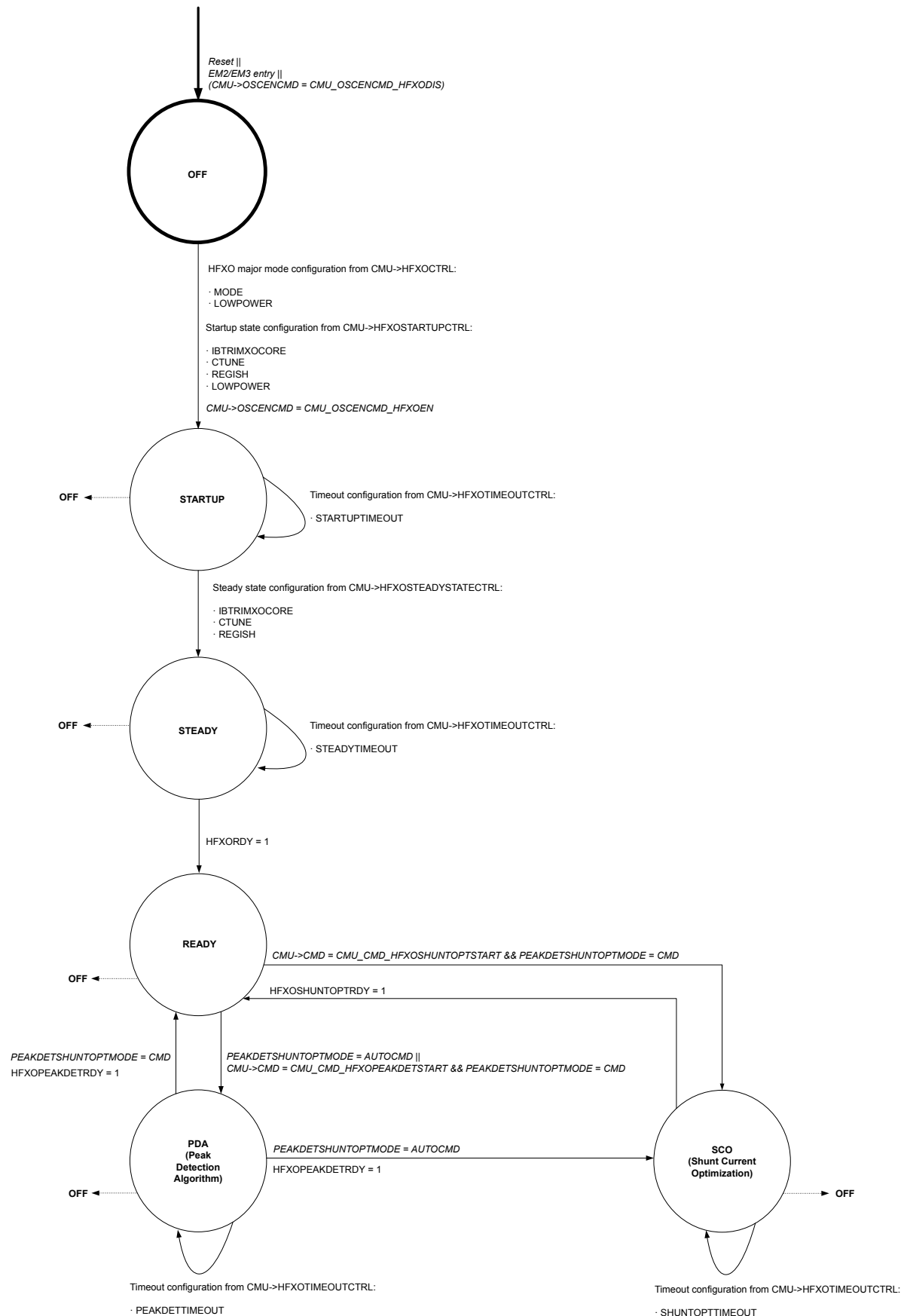
Figure 11.7. CMU HFXO control state machine
