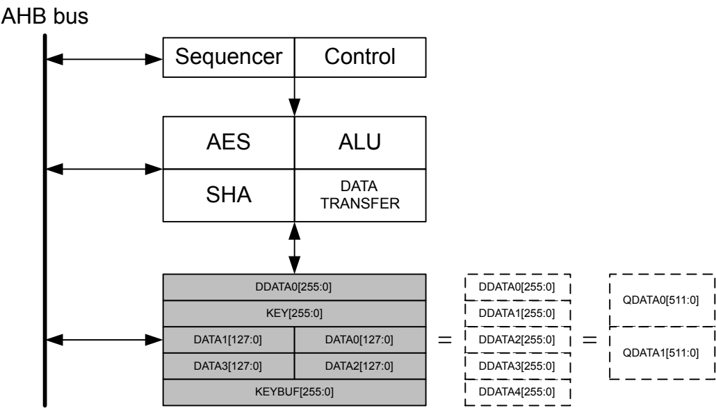
Figure 31.1. CRYPTO Overview
