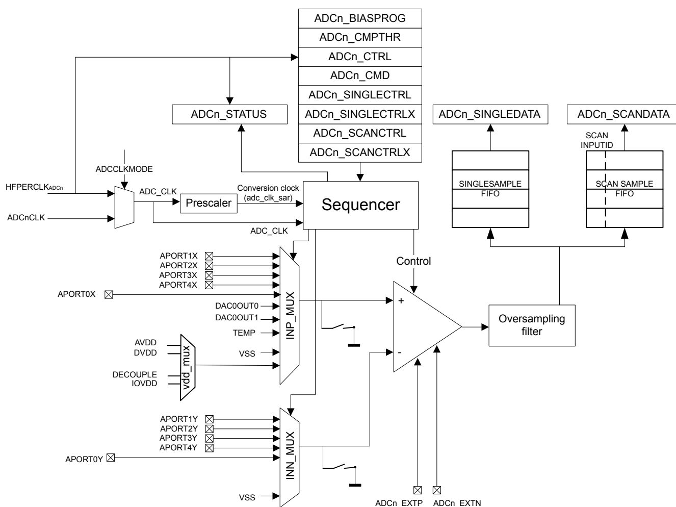
Figure 26.1. ADC Overview
