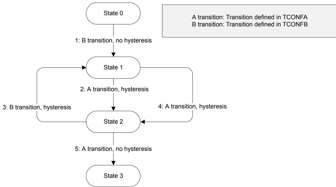
Figure 28.13. Decoder hysteresis
