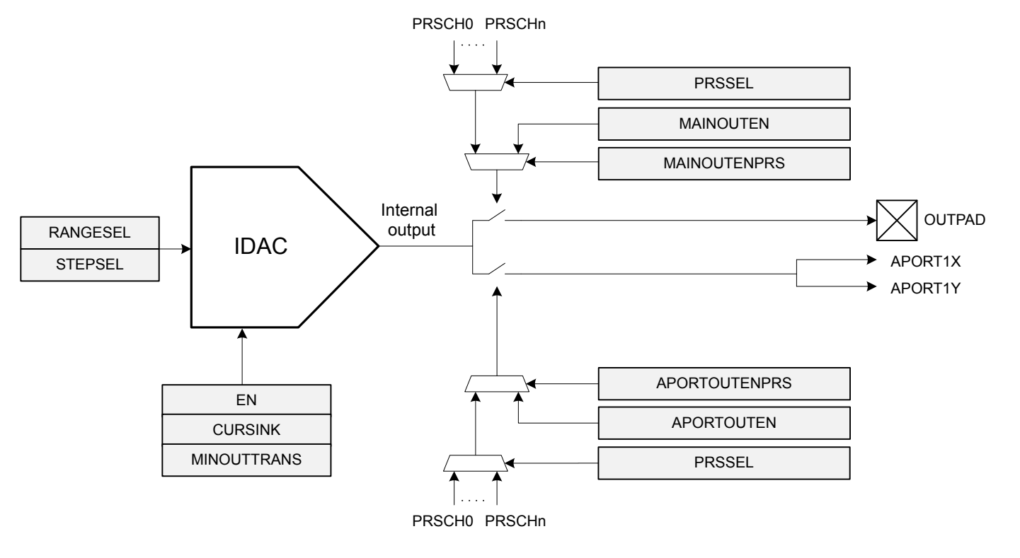
Figure 27.1. IDAC Overview
