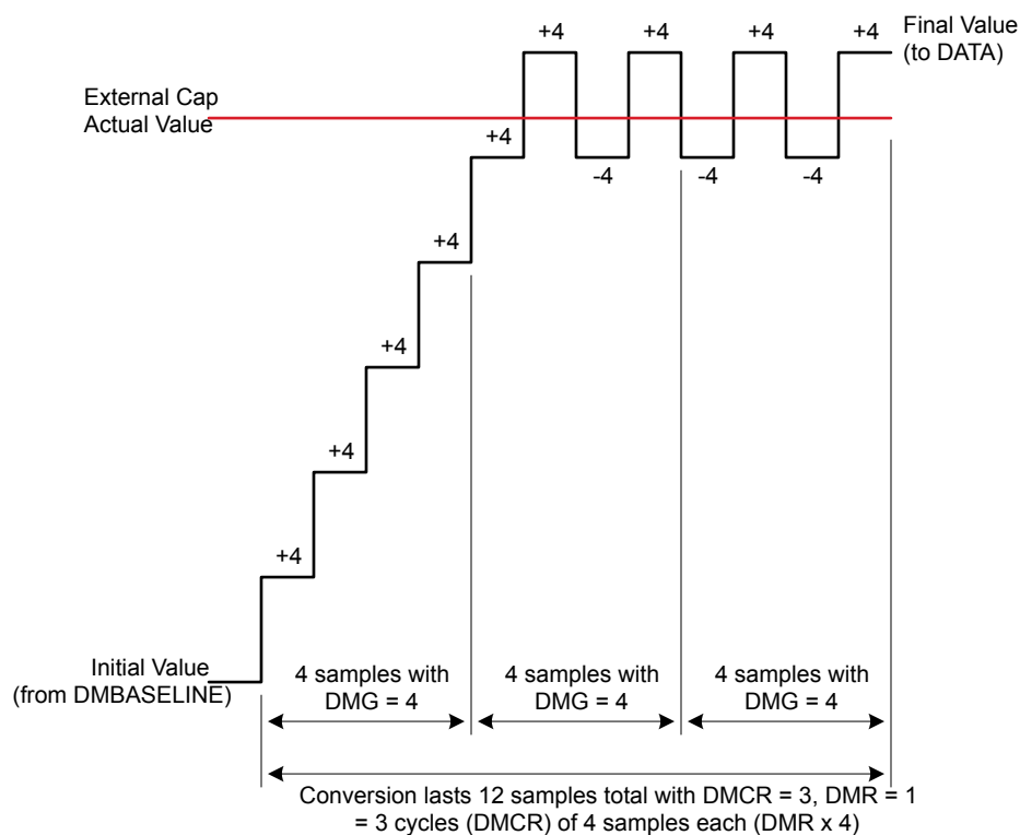
Figure 34.3. Delta modulation conversion with fixed delta step (DMGDIS = 1)
