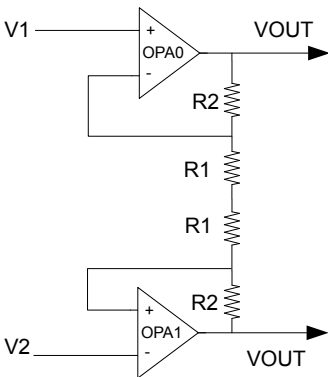
Figure 24.11. Instrumentaion Amplifier Overview
