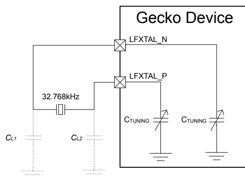
Figure 11.8. LFXO Pin Connection
