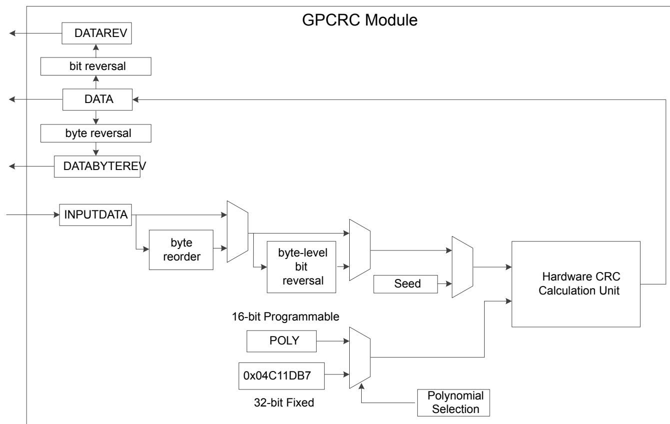
Figure 29.1. GPCRC Overview
