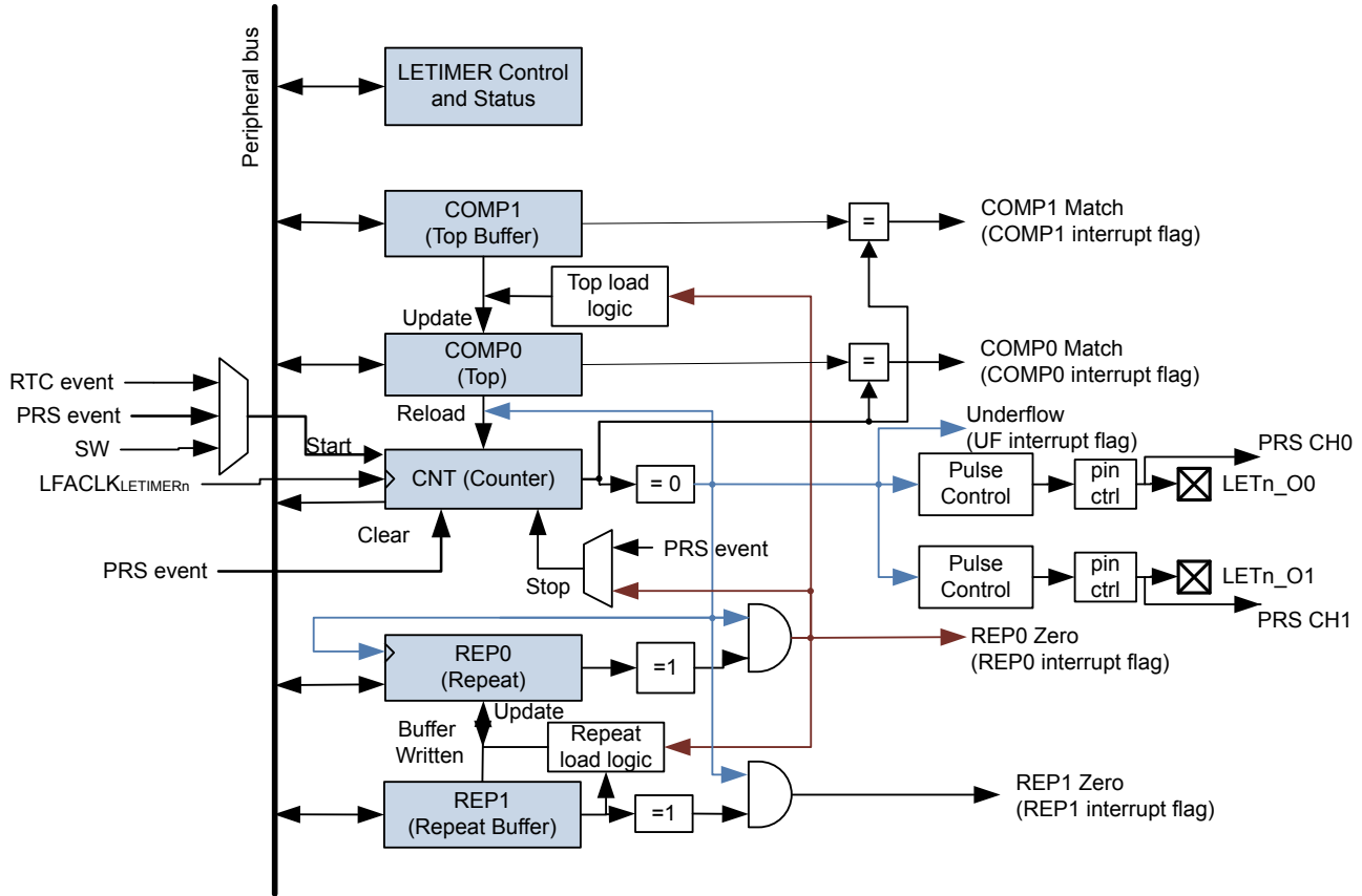
Figure 21.1. LETIMER Overview
