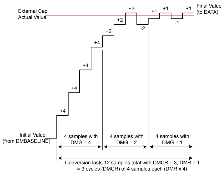
Figure 34.2. Delta modulation conversion with gain reduction (DMGRDIS = 0)
