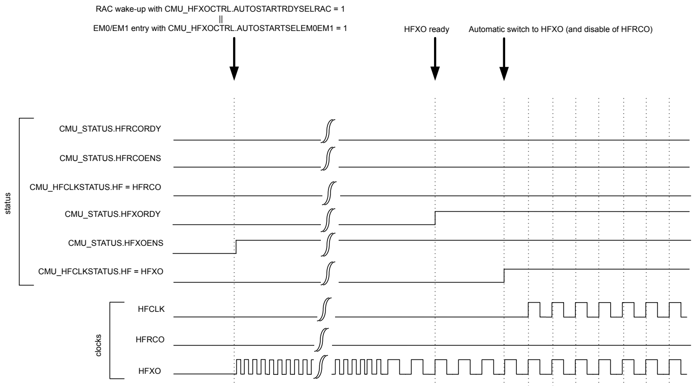
Figure 11.13. CMU Automatic startup and selection of HFXO
