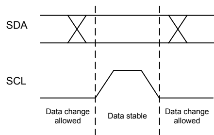
Figure 17.5. I2C Bit Transfer on I 2 C-Bus
