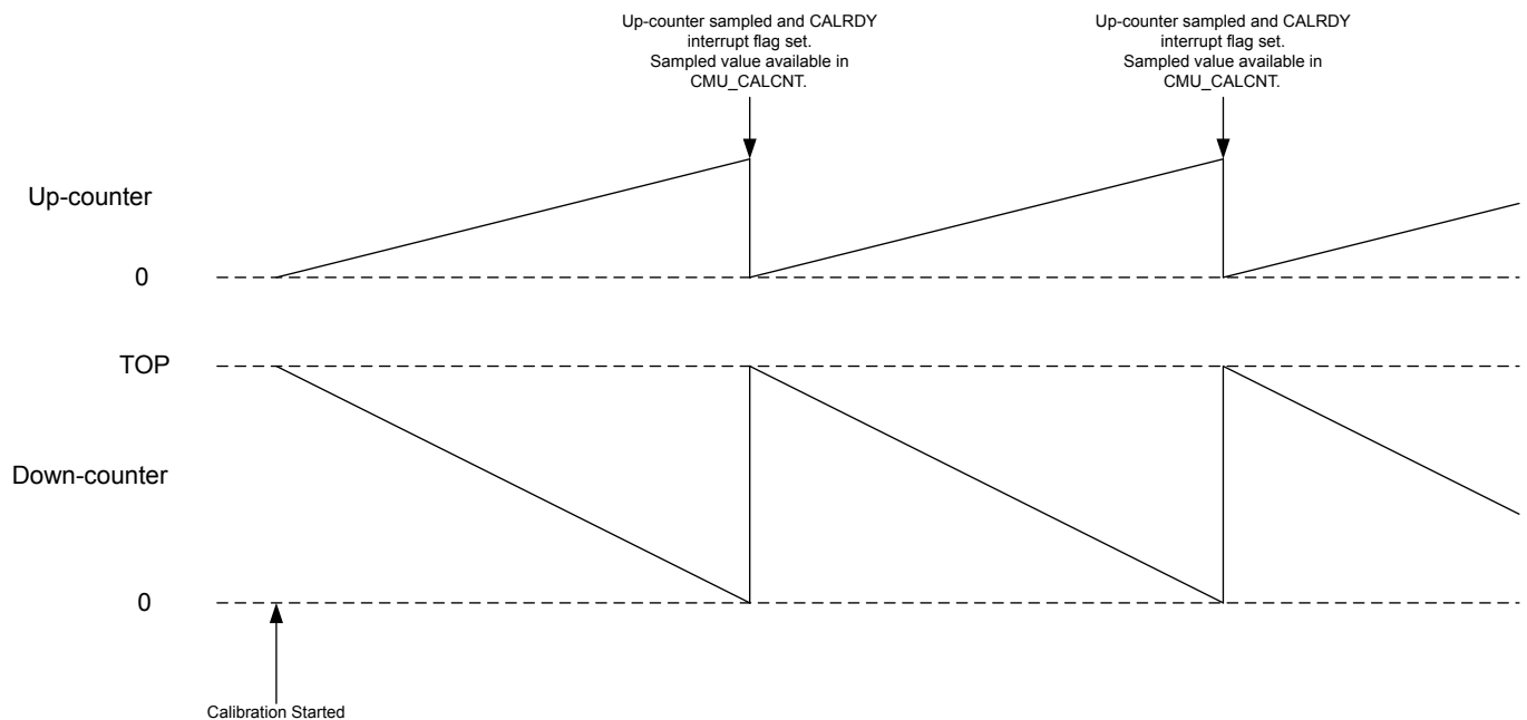
Figure 11.12. Continuous Calibration (CONT=1)
