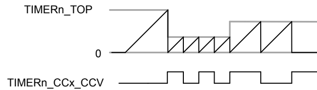
Figure 20.17. TIMER/WTIMER Up-count Frequency Generation
