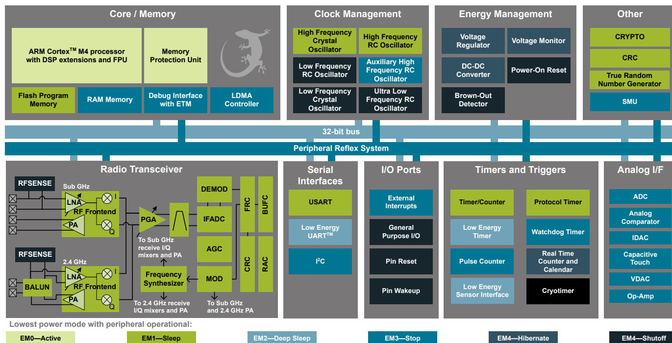
Figure 2.1. EFR32xG12 Wireless Gecko System-On-Chip Block Diagram
