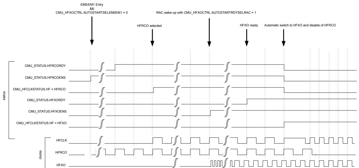
Figure 11.15. CMU Automatic HFXO startup/selection while HFRCO started/selected
