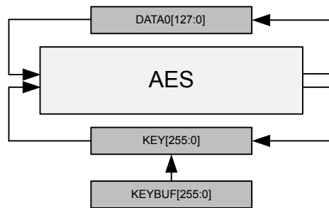
Figure 31.3. CRYPTO AES Overview
