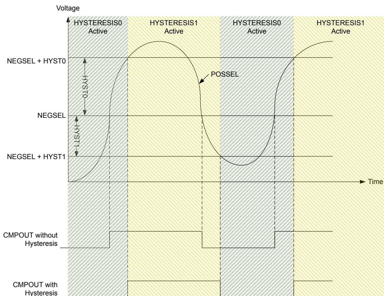
Figure 25.3. Hysteresis
