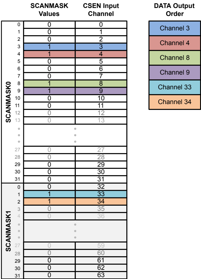
Figure 34.4. Scan Mode Sequencing
