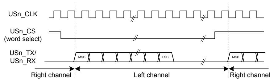
Figure 18.22. USART Standard I2S waveform (reduced accuracy)
