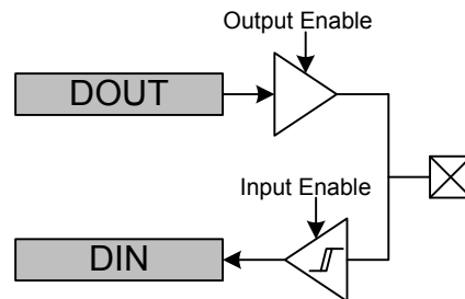
Figure 32.3. Push-Pull Configuration
