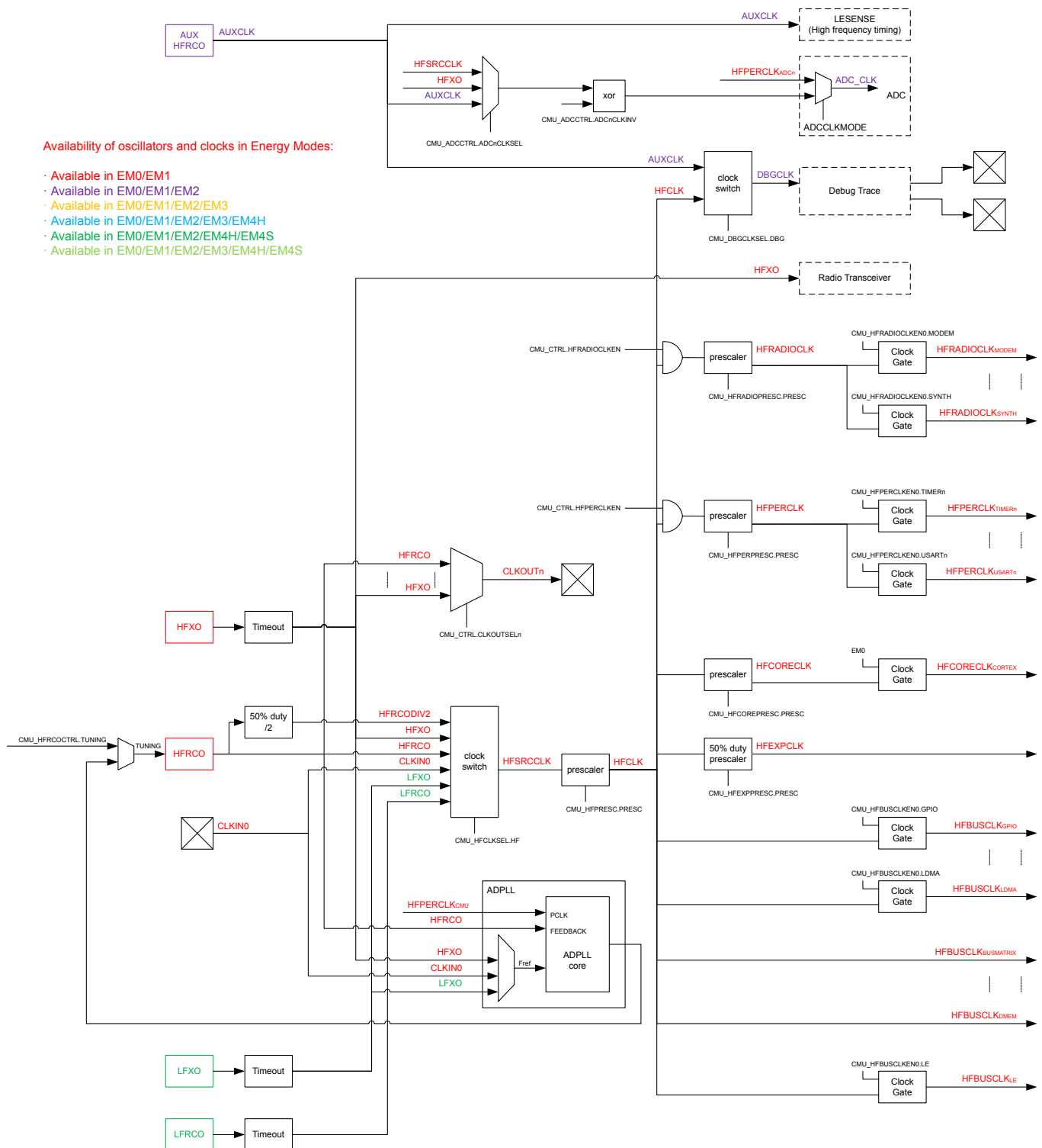
Figure 11.1. CMU Overview - High Frequency Portion
