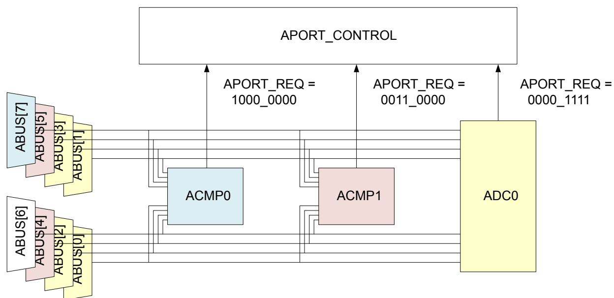
Figure 33.4. APORT Example 1
