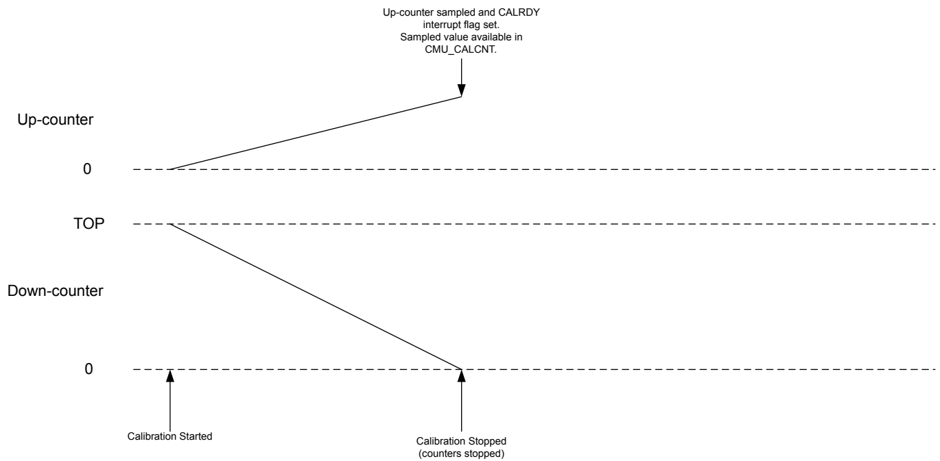
Figure 11.11. Single Calibration (CONT=0)
