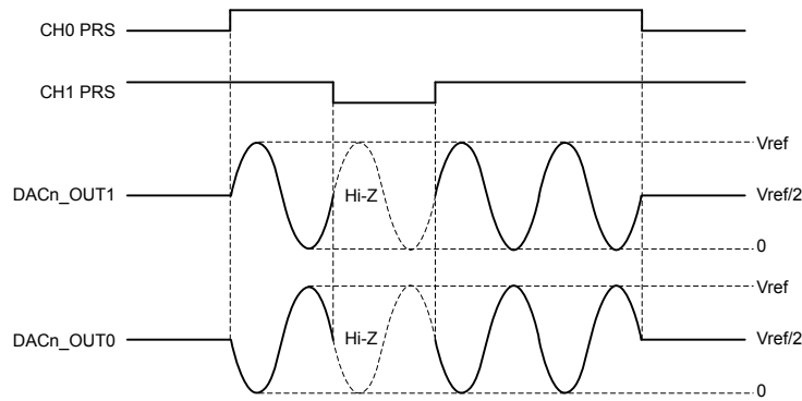
Figure 23.6. VDAC Sine Mode
