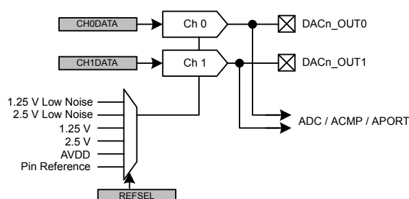
Figure 23.1. VDAC Overview
