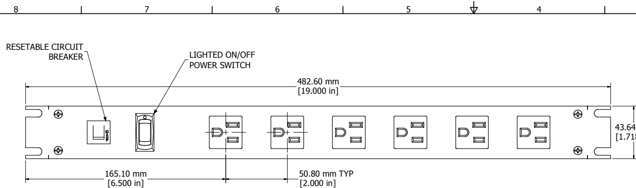
ASSEMBLY - VIEW FROM FRONT
