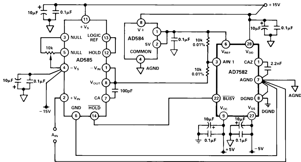
Figure 23. AD7582-AD585 Interface
