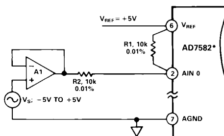
Figure 14. Bipolar -5V to +5V Operation
