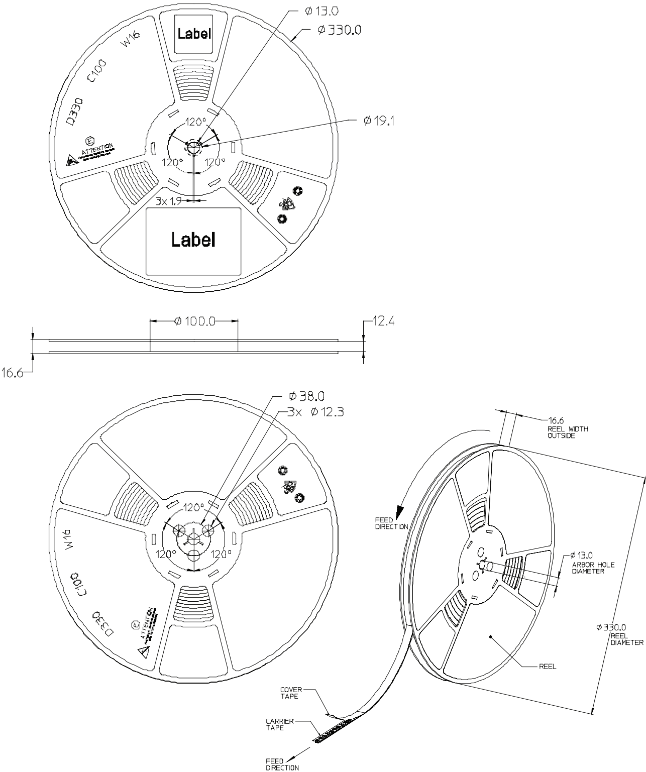
Figure 11. Emitter reel packaging.
