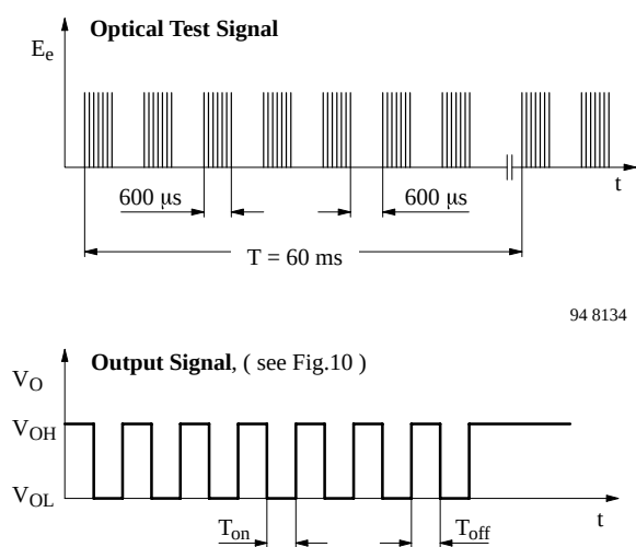
Figure 8. Output Function
