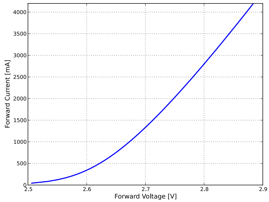
Figure 5c: Typical forward current vs. forward voltage for LXR-Qxxx at T_j = 85^\circ\text{C} .
