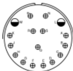
Insert Arrangement 36-13 Service Rating N, P, Q = E; Bal. = A Number of Contacts 2 15 Contact Size 12 16
