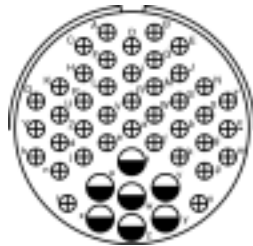
Insert Arrangement 36-7 Service Rating A Number of Contacts 7 40 Contact Size 12 16
