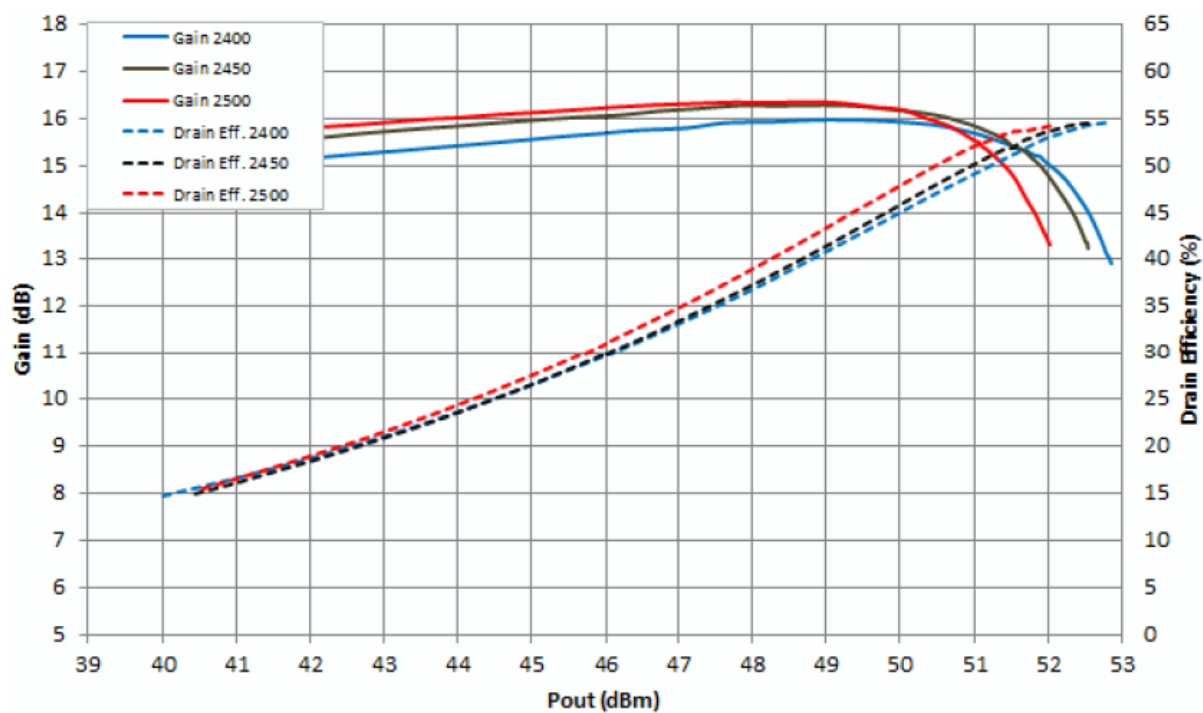
Figure 2. Power gain and drain efficiency vs output power (2400 - 2500 MHz)
