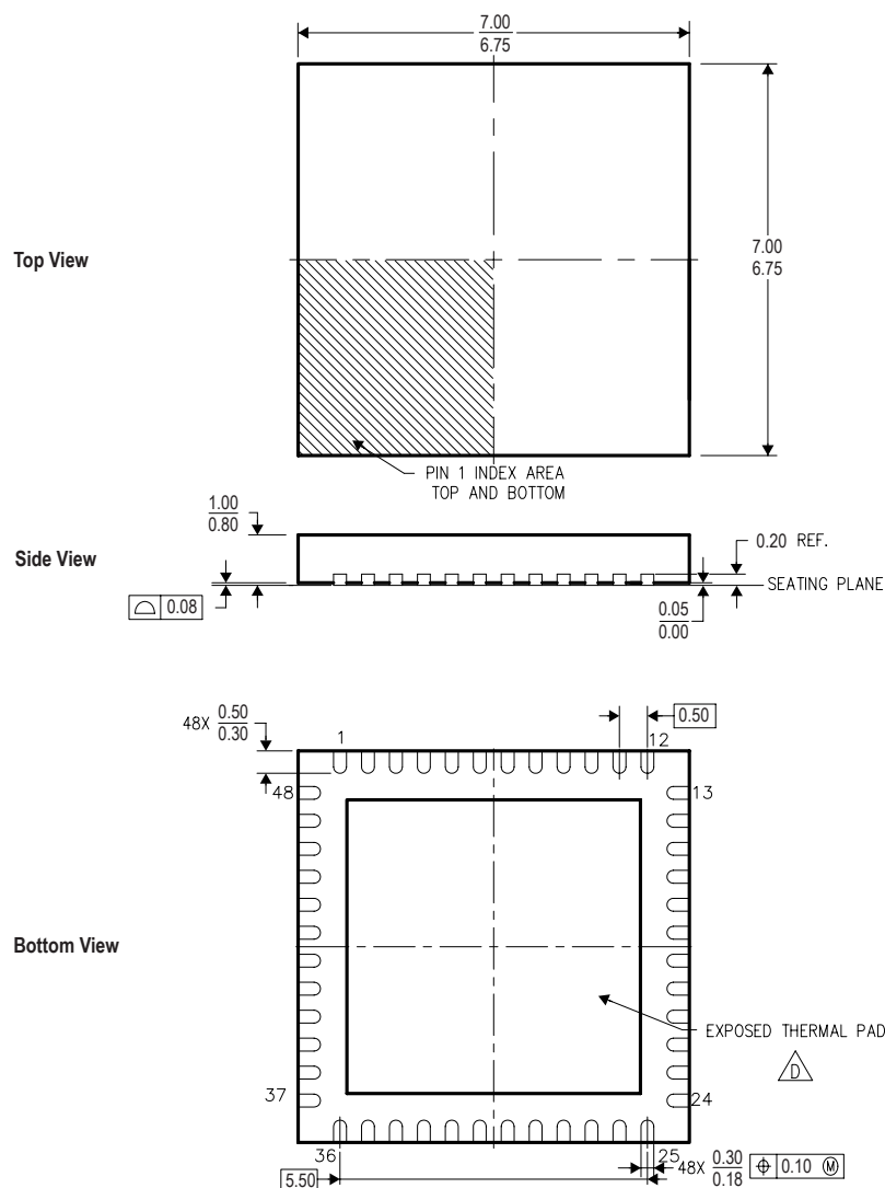
Figure D-4. Stellaris LM3S301 48-Pin QFN Package
