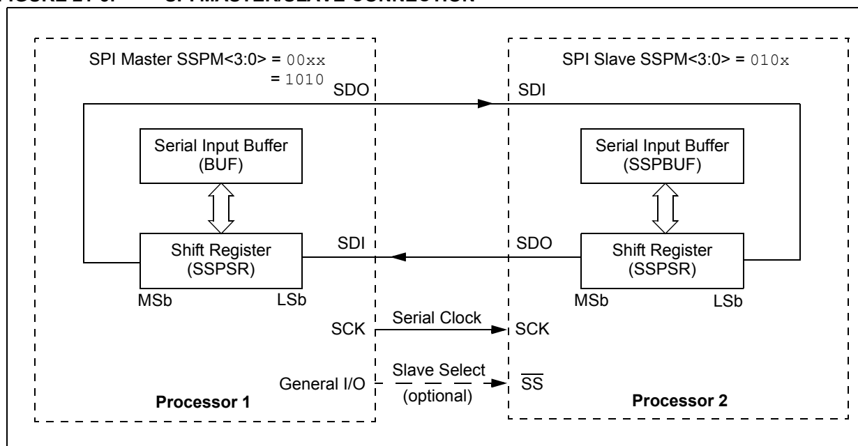
FIGURE 21-5: SPI MASTER/S�AVE CONNECTION
