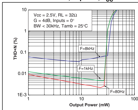
Figure 26. THD+N vs. output power RL = 32\ \Omega , in-phase, V_{CC} = 2.5\ V
