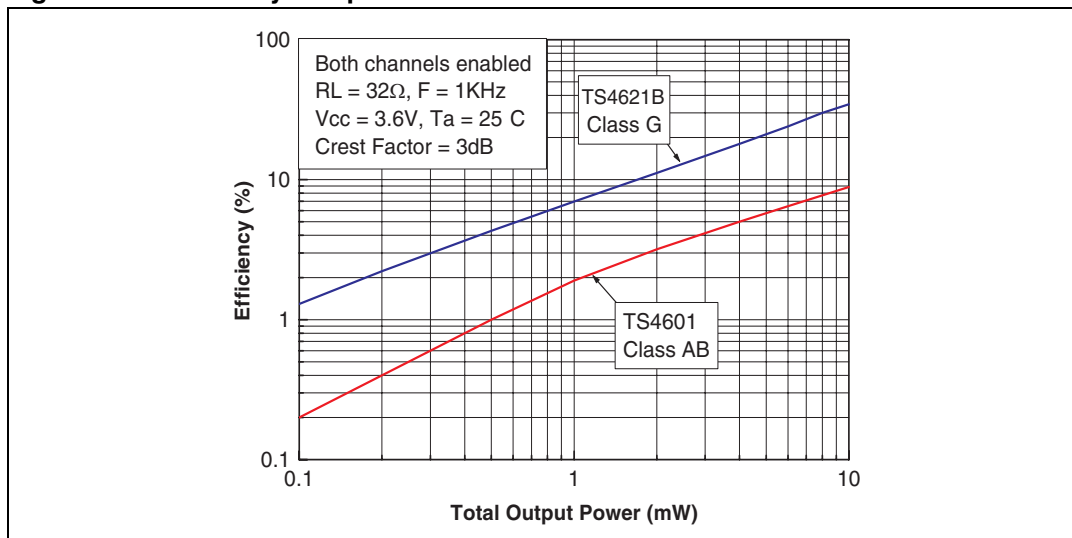
Figure 76. Efficiency comparison
