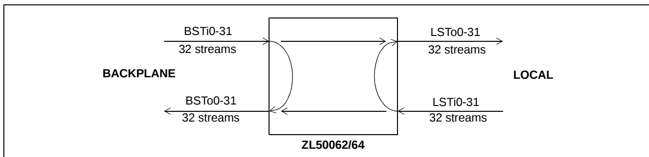
Figure 5 - 8,192 x 8,192 Channels (16Mbps), Bi-directional Switching
