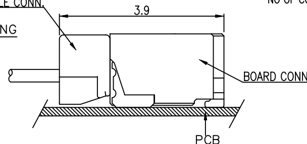
MATED CONDITION
