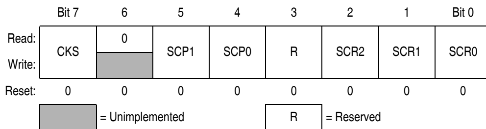
Figure 13-19. SCI Baud Rate Register (SCBR)
