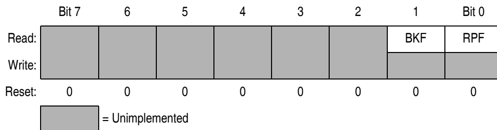
Figure 13-17. SCI Status Register 2 (SCS2)
