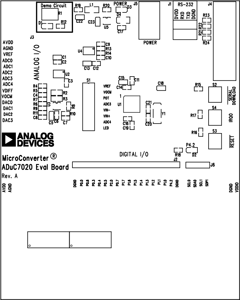
ADuC7020 EVALUATION BOARD Rev. A- Component Side View Silkscreen Top
