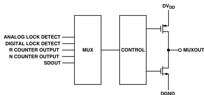
Figure 25. MUXOUT Circuit
