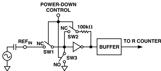
Figure 21. Reference Input Stage
