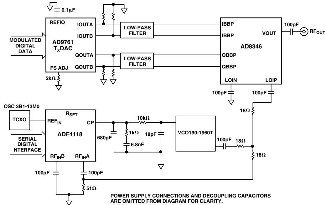
Figure 28. Direct Conversion Transmitter Solution
